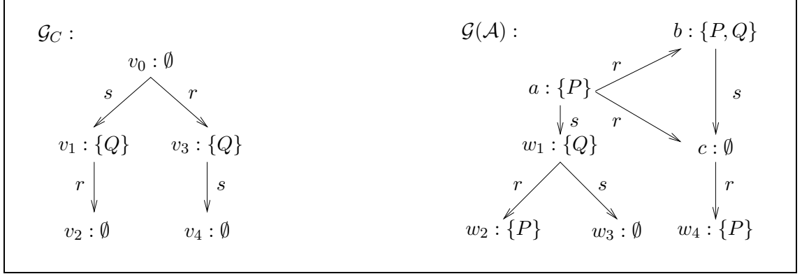
Figure 5: The \mathcal{EL} description tree of C and the \mathcal{EL} description graph of \mathcal{A} .
