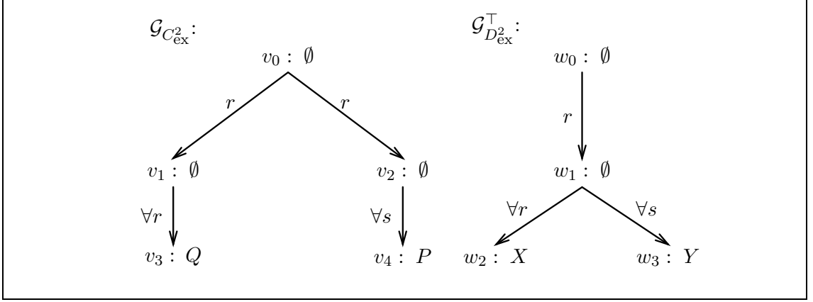
Figure 9: The description trees for C_{ex}^2 and D_{ex}^2 .
