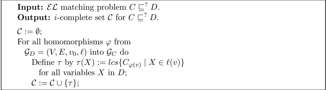
Figure 8: The \mathcal{EL} matching algorithm
