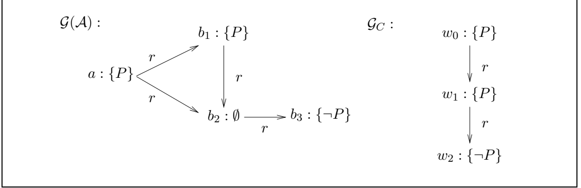
Figure 6: The \mathcal{EL}_\neg description graph and the \mathcal{EL}_\neg description tree of our example.
